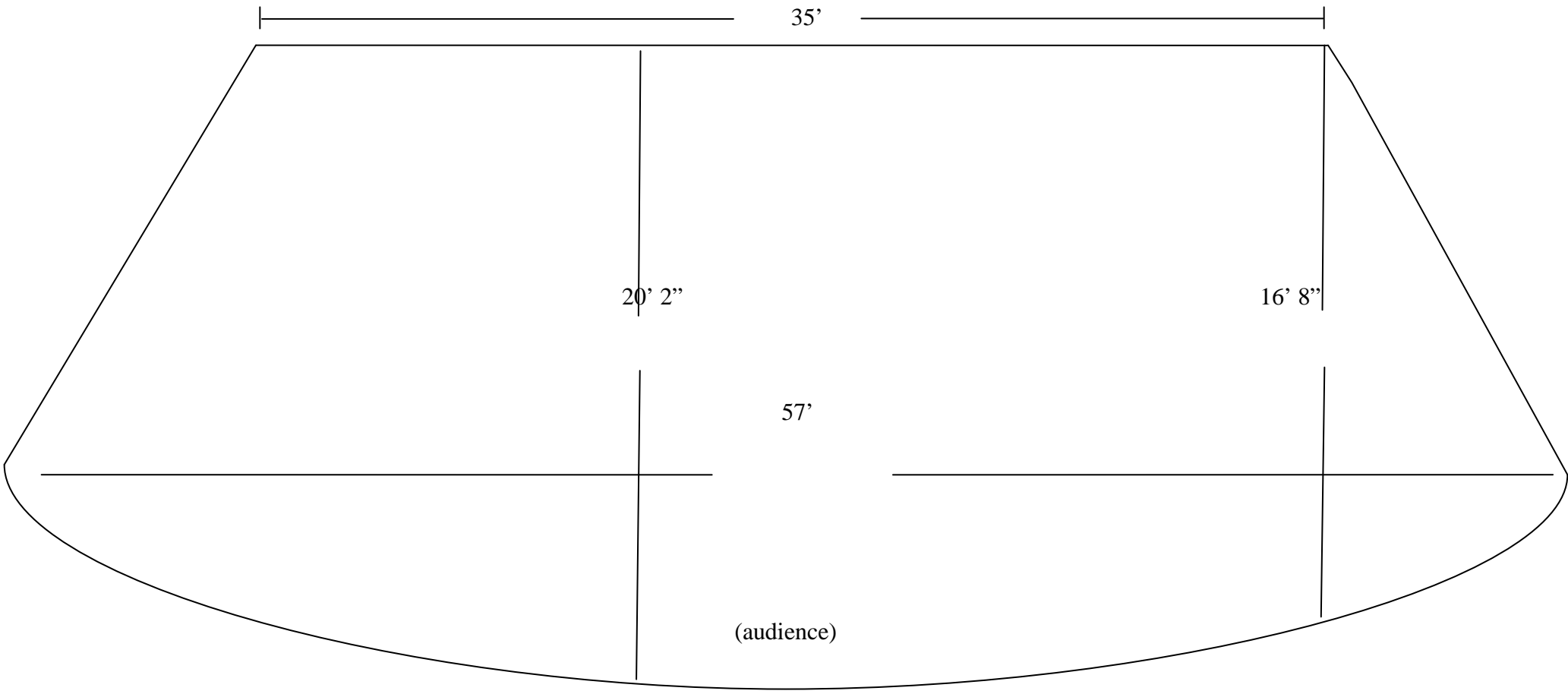
Merkin Hall stage dimensions (From balcony skirt to upstage wall = 54')
